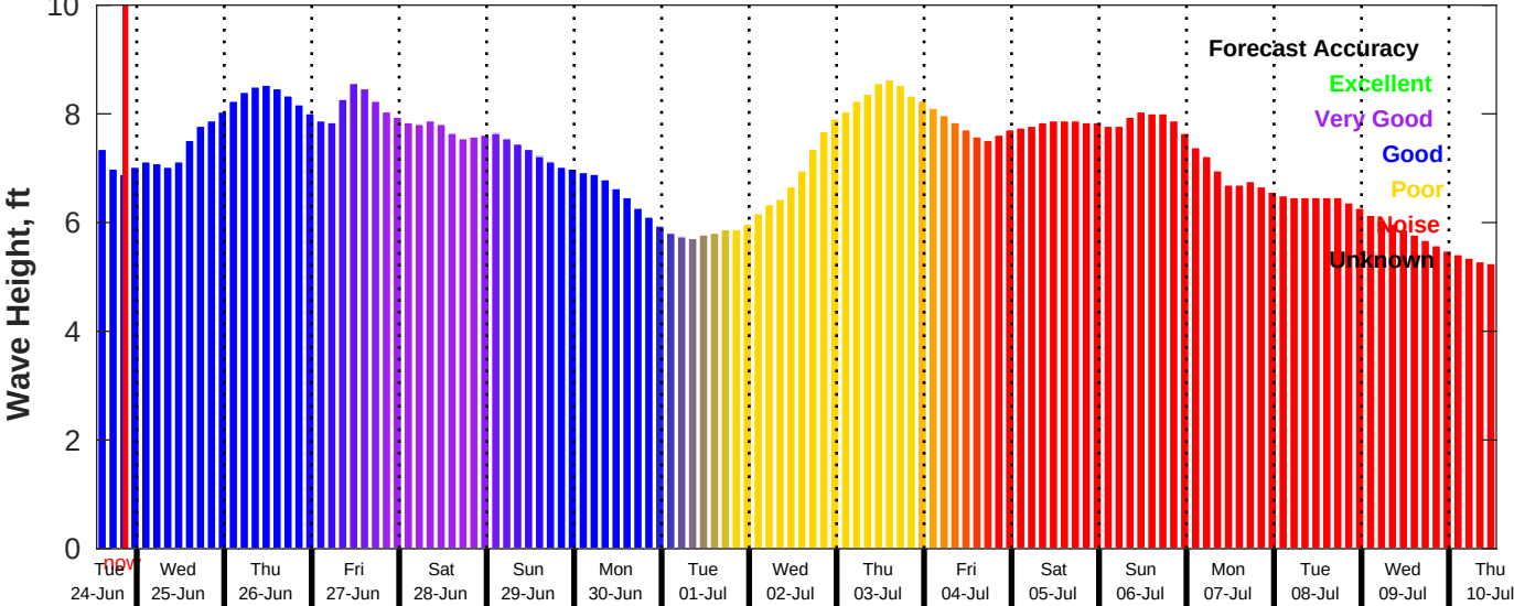
GFS Wave Forecast for NDBC 51209 from 24-Jun-2025 13:00:00 to 10-Jul-2025 13:00:00
