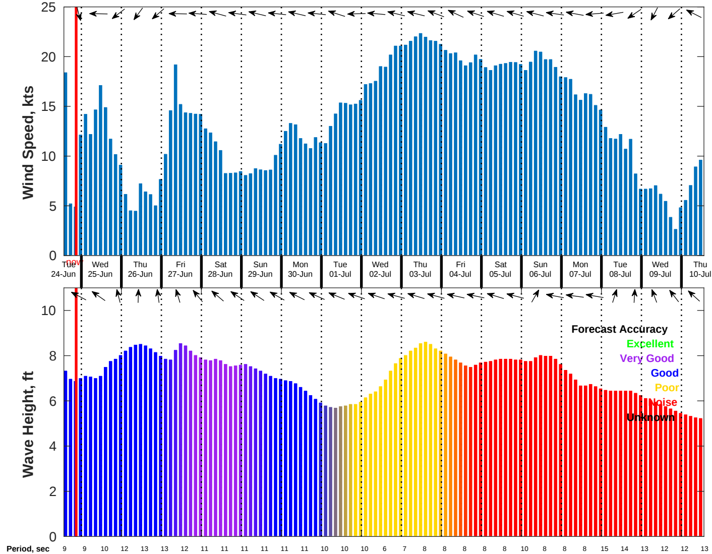
Wind & Wave Forecast for NDBC 51209 from 24-Jun-2025 13:00:00 to 10-Jul-2025 13:00:00
