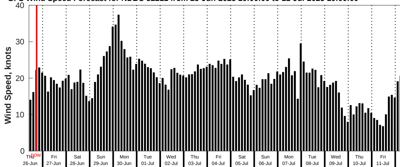
GFS Wind Speed Forecast for NDBC 52211 from 25-Jun-2025 10:00:00 to 11-Jul-2025 10:00:00
