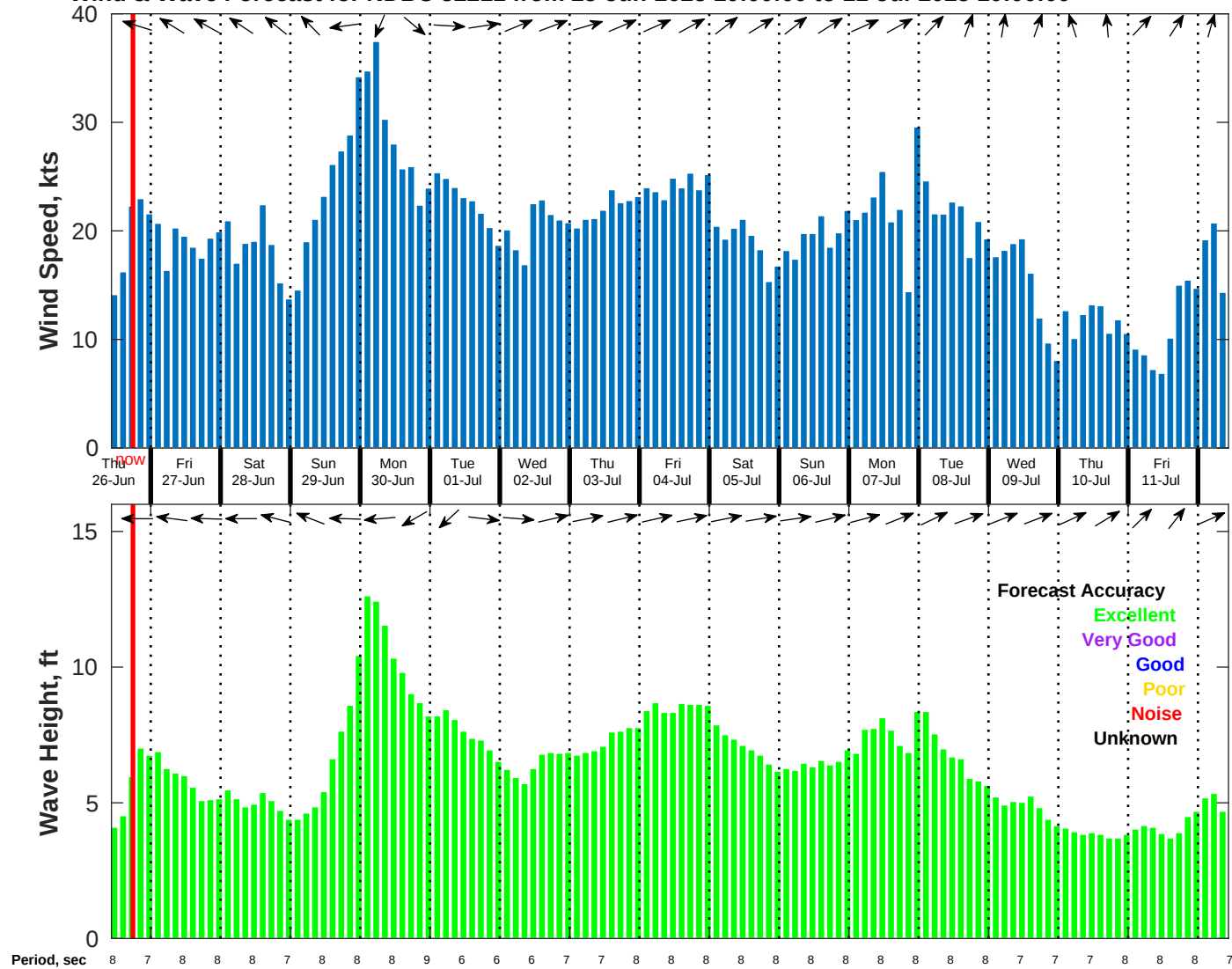
Wind & Wave Forecast for NDBC 52211 from 25-Jun-2025 10:00:00 to 11-Jul-2025 10:00:00
