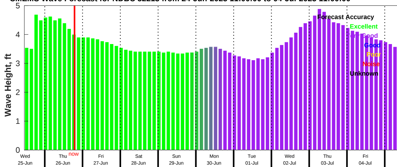
CMEMS Wave Forecast for NDBC 52213 from 24-Jun-2025 11:00:00 to 04-Jul-2025 11:00:00
