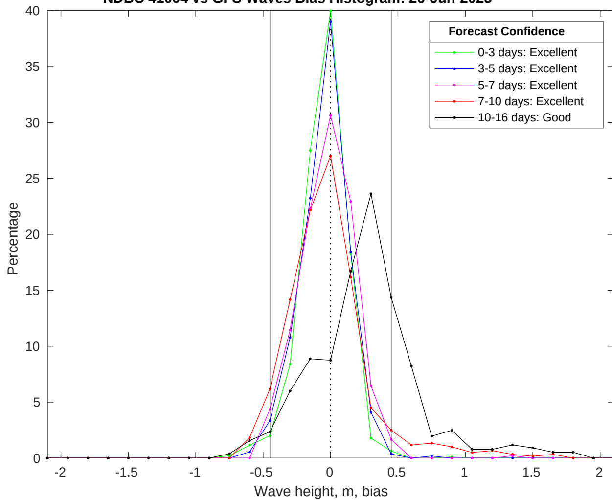
NDBC 41004 vs GFS Waves Bias Histogram: 26-Jun-2025
