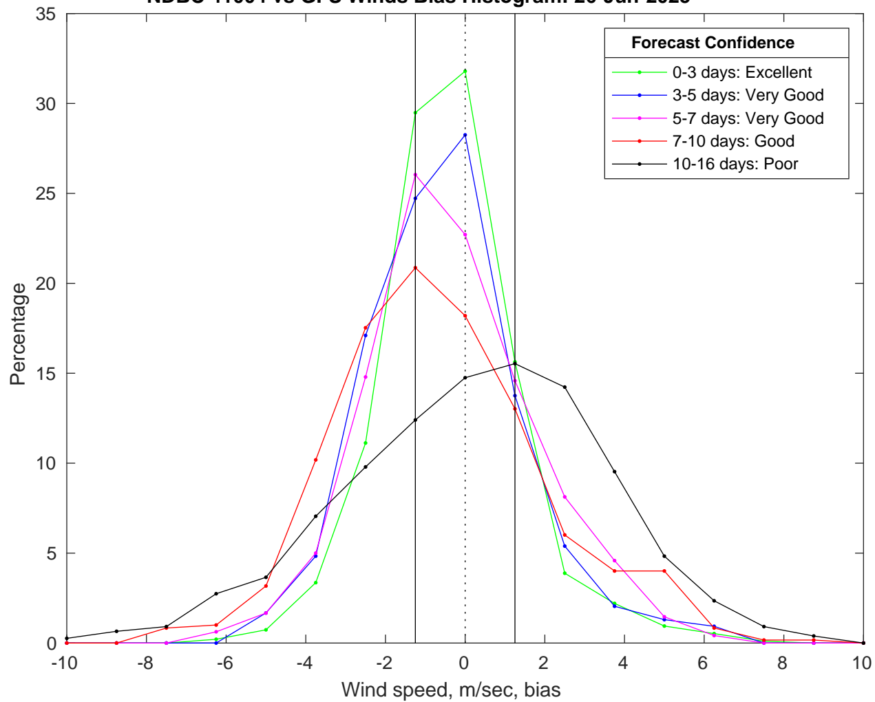
NDBC 41004 vs GFS Winds Bias Histogram: 26-Jun-2025
