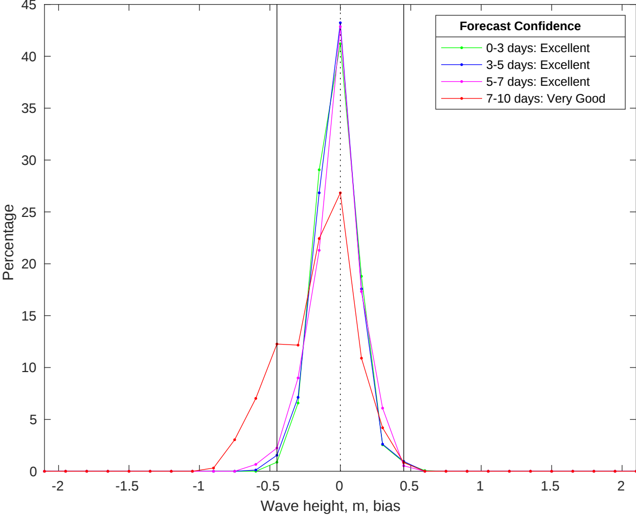
NDBC 41013 vs CMEMS Waves Bias Histogram: 26-Jun-2025
