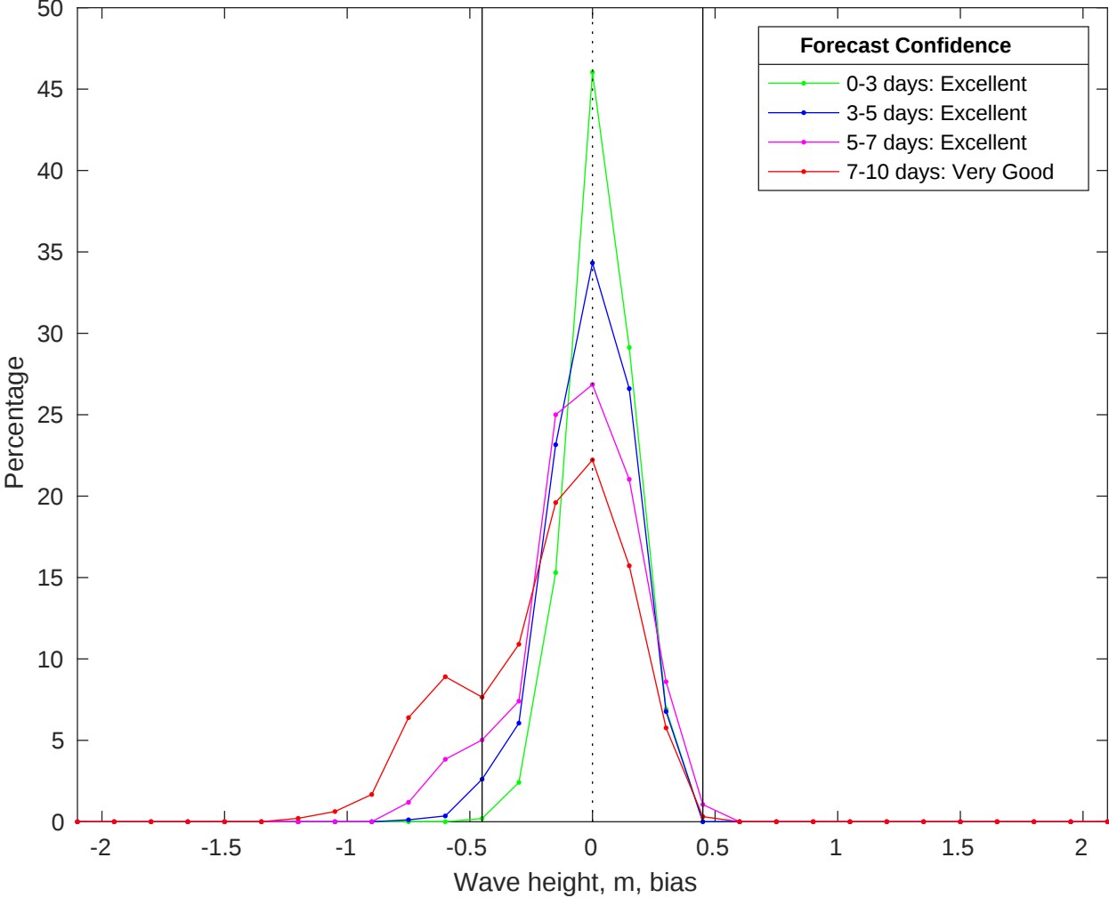
NDBC 41040 vs CMEMS Waves Bias Histogram: 26-Jun-2025
