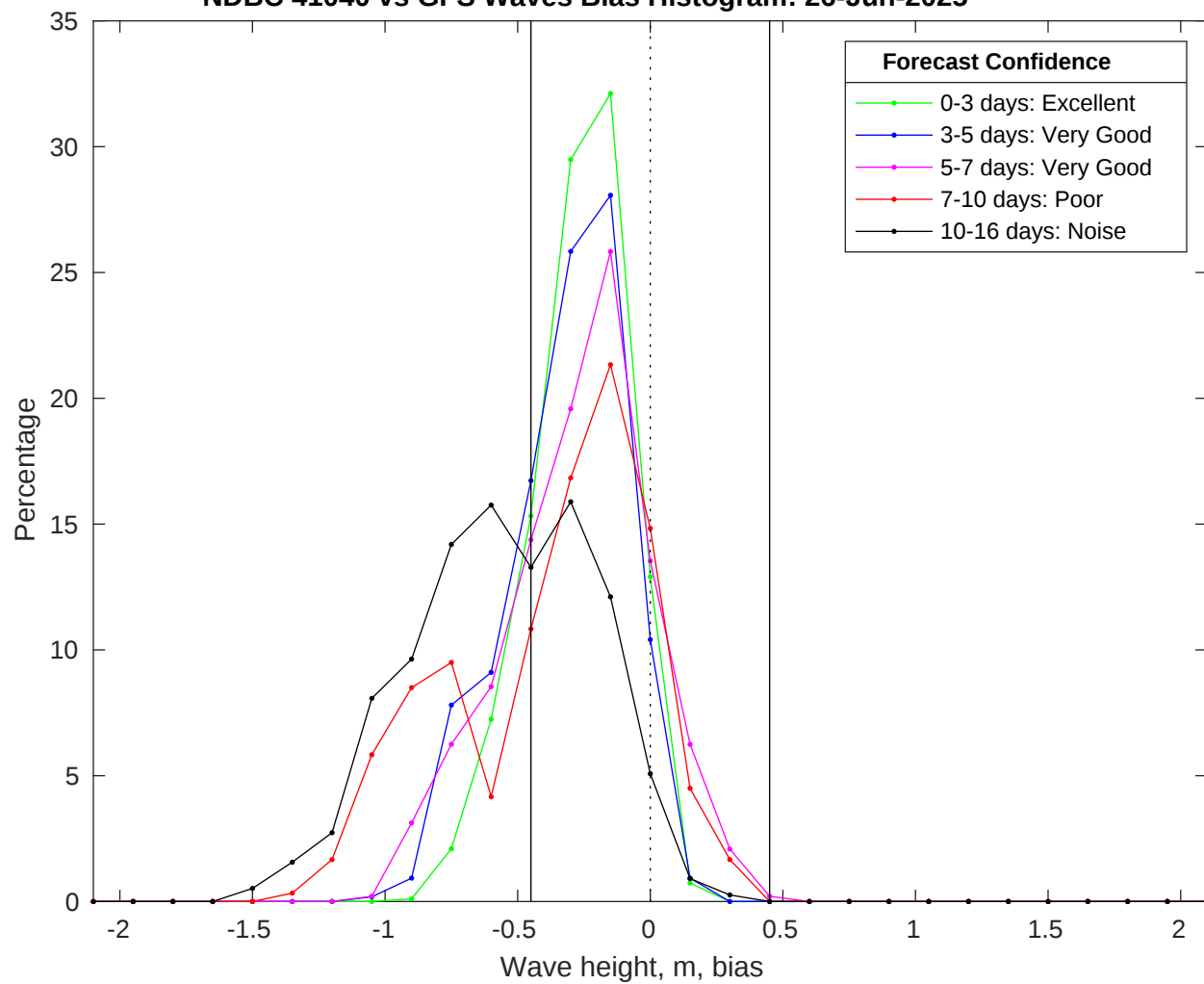
NDBC 41040 vs GFS Waves Bias Histogram: 26-Jun-2025
