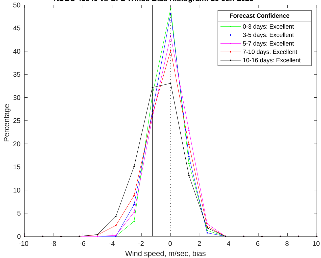
NDBC 41040 vs GFS Winds Bias Histogram: 26-Jun-2025
