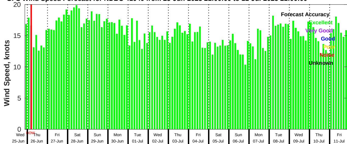
GFS Wind Speed Forecast for NDBC 41040 from 25-Jun-2025 21:00:00 to 11-Jul-2025 21:00:00
