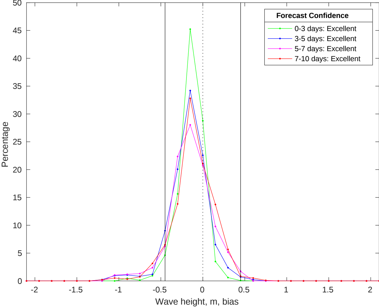
NDBC 42019 vs CMEMS Waves Bias Histogram: 26-Jun-2025
