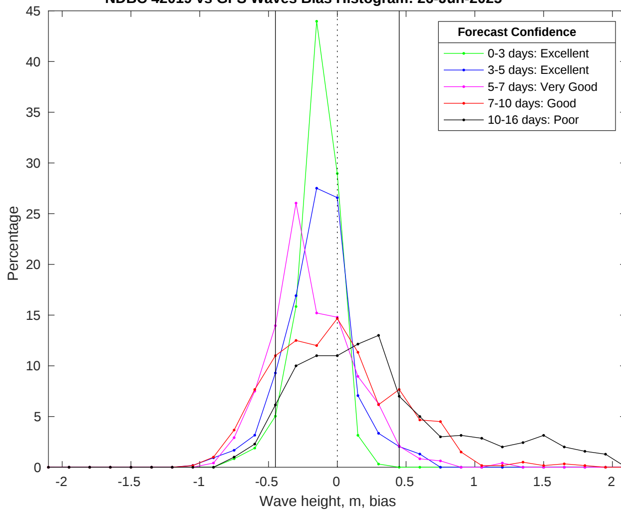
NDBC 42019 vs GFS Waves Bias Histogram: 26-Jun-2025
