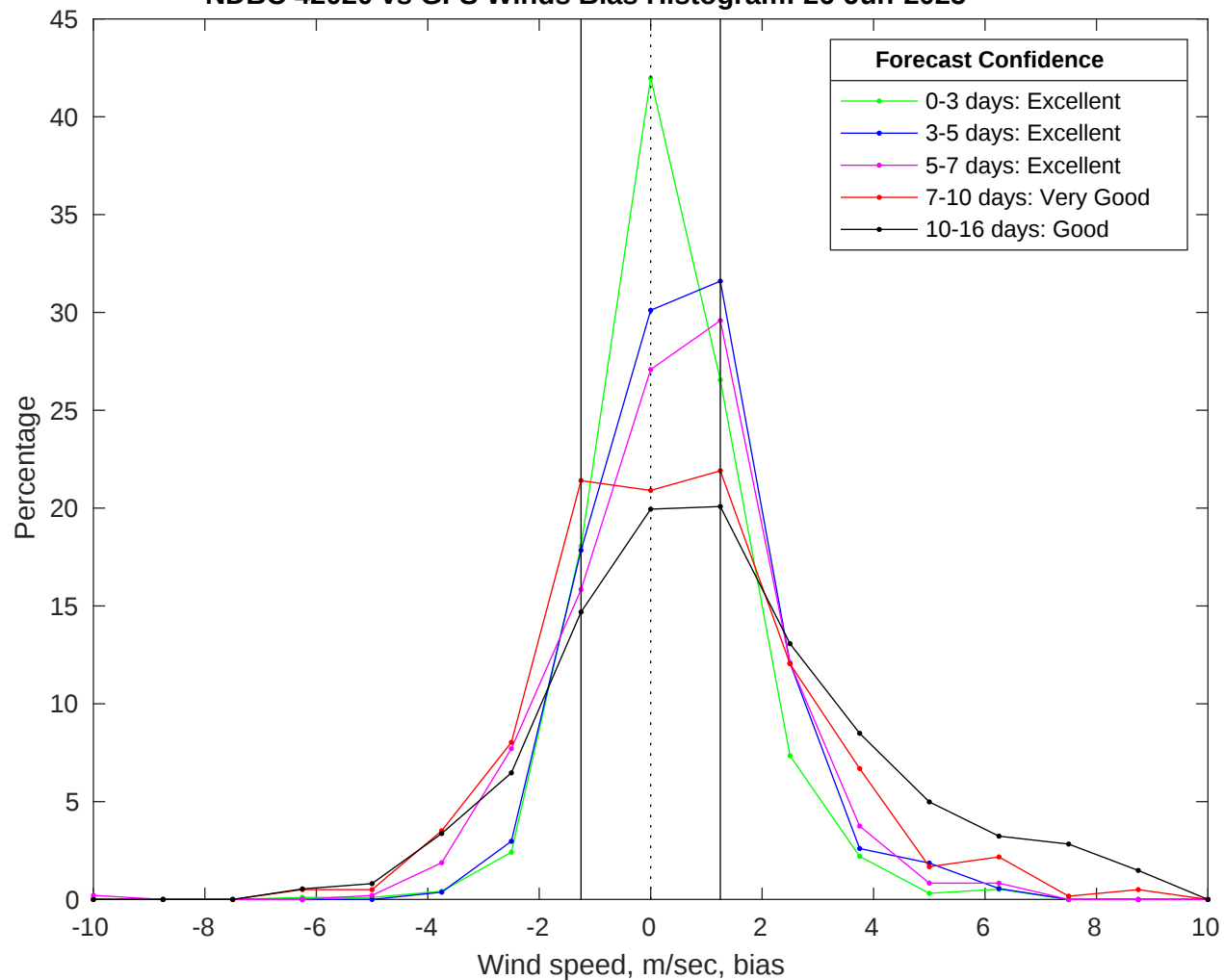
NDBC 42020 vs GFS Winds Bias Histogram: 26-Jun-2025
