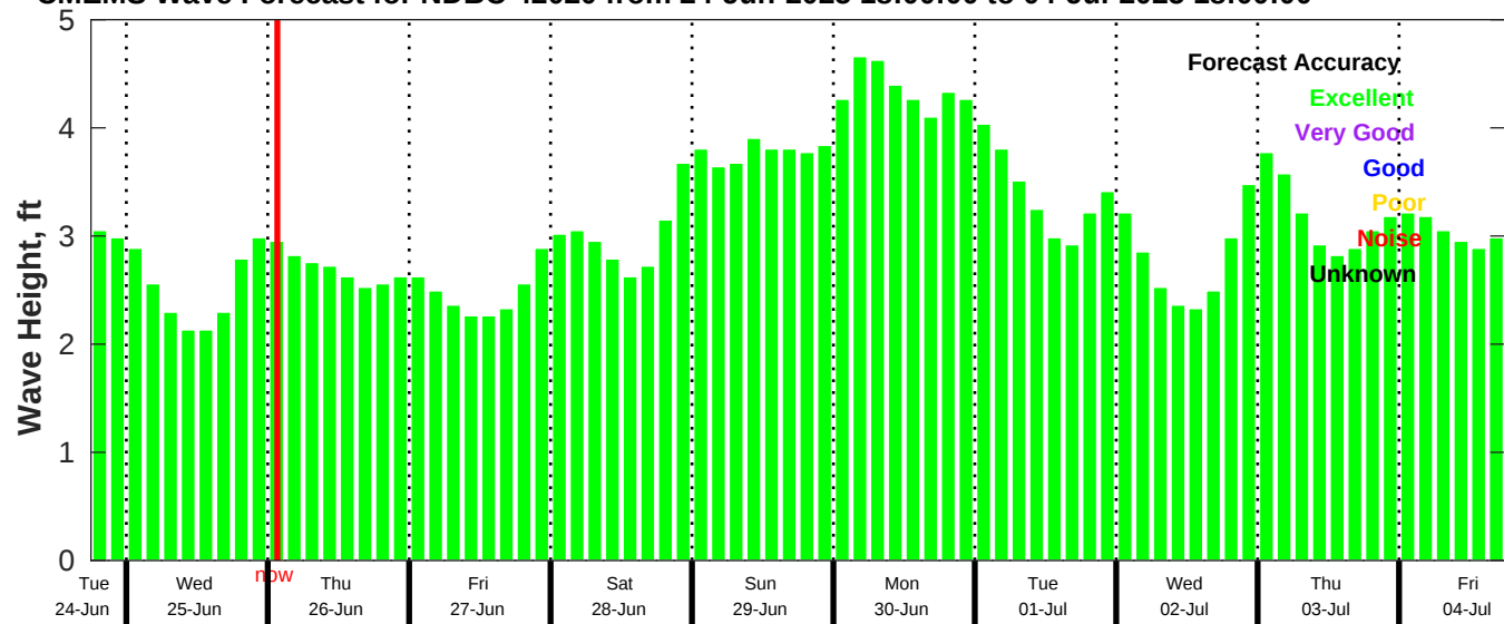
CMEMS Wave Forecast for NDBC 42020 from 24-Jun-2025 18:00:00 to 04-Jul-2025 18:00:00
