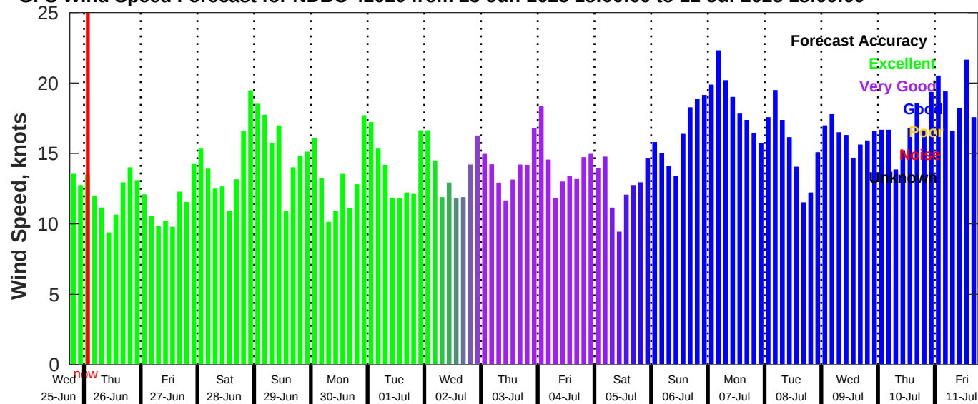
GFS Wind Speed Forecast for NDBC 42020 from 25-Jun-2025 18:00:00 to 11-Jul-2025 18:00:00
