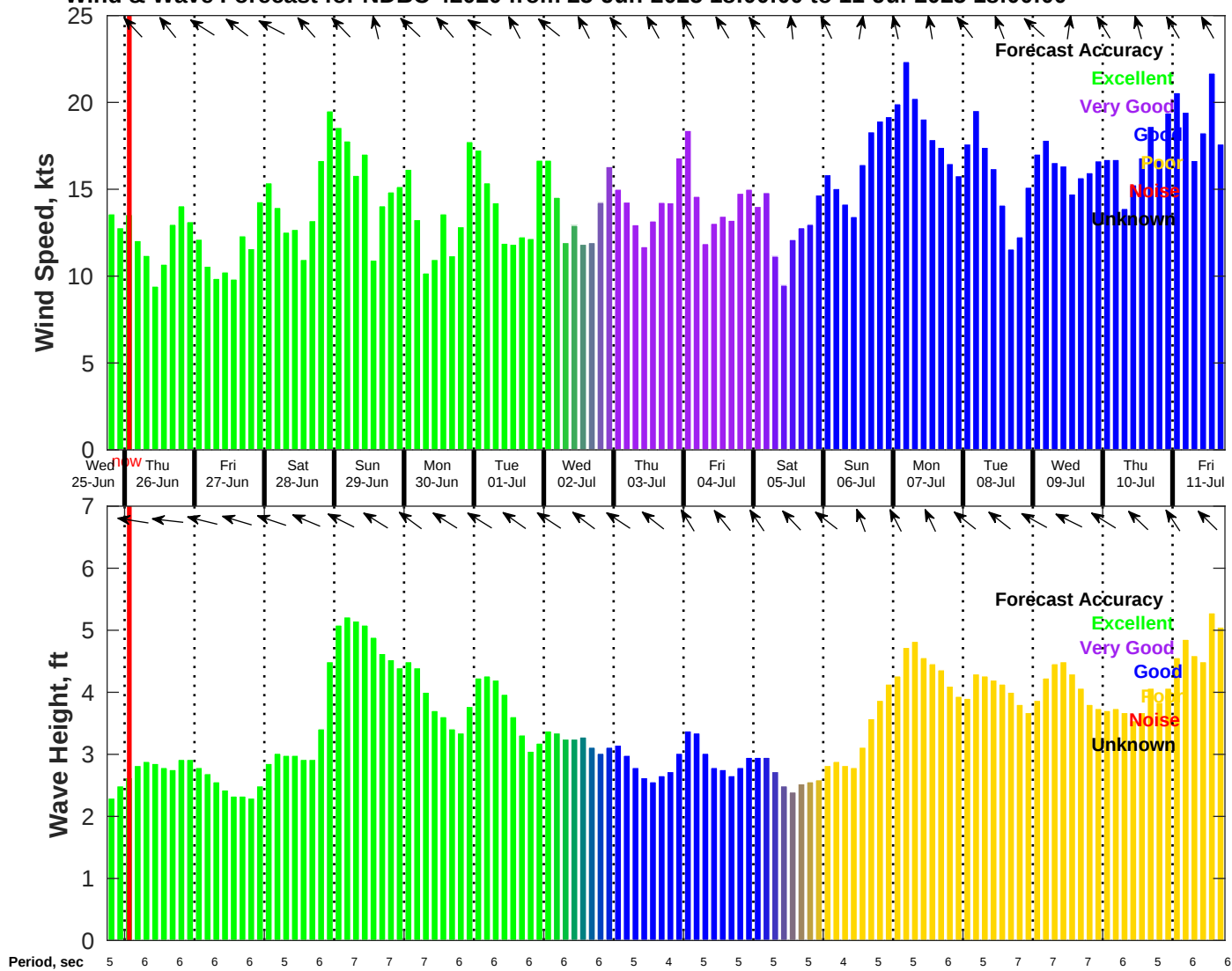
Wind & Wave Forecast for NDBC 42020 from 25-Jun-2025 18:00:00 to 11-Jul-2025 18:00:00
