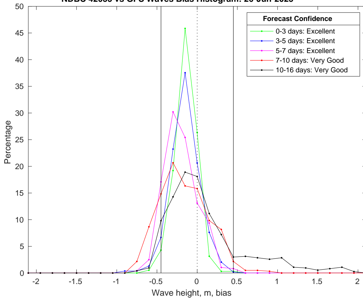
NDBC 42035 vs GFS Waves Bias Histogram: 26-Jun-2025
