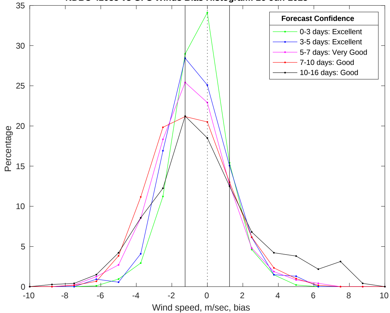
NDBC 42035 vs GFS Winds Bias Histogram: 26-Jun-2025
