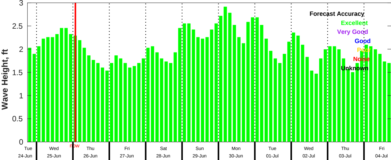
CMEMS Wave Forecast for NDBC 42035 from 24-Jun-2025 18:00:00 to 04-Jul-2025 18:00:00
