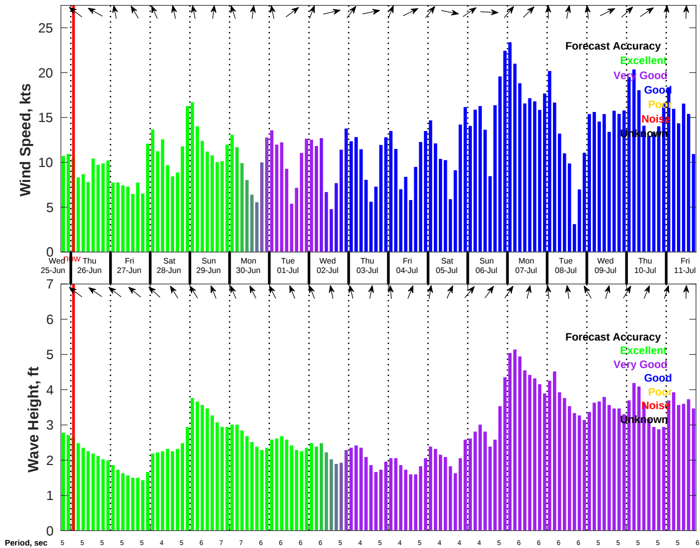
Wind & Wave Forecast for NDBC 42035 from 25-Jun-2025 18:00:00 to 11-Jul-2025 18:00:00
