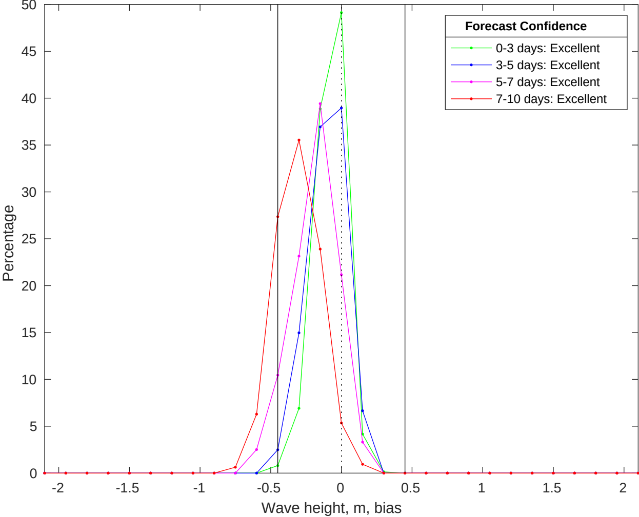
NDBC 42036 vs CMEMS Waves Bias Histogram: 26-Jun-2025
