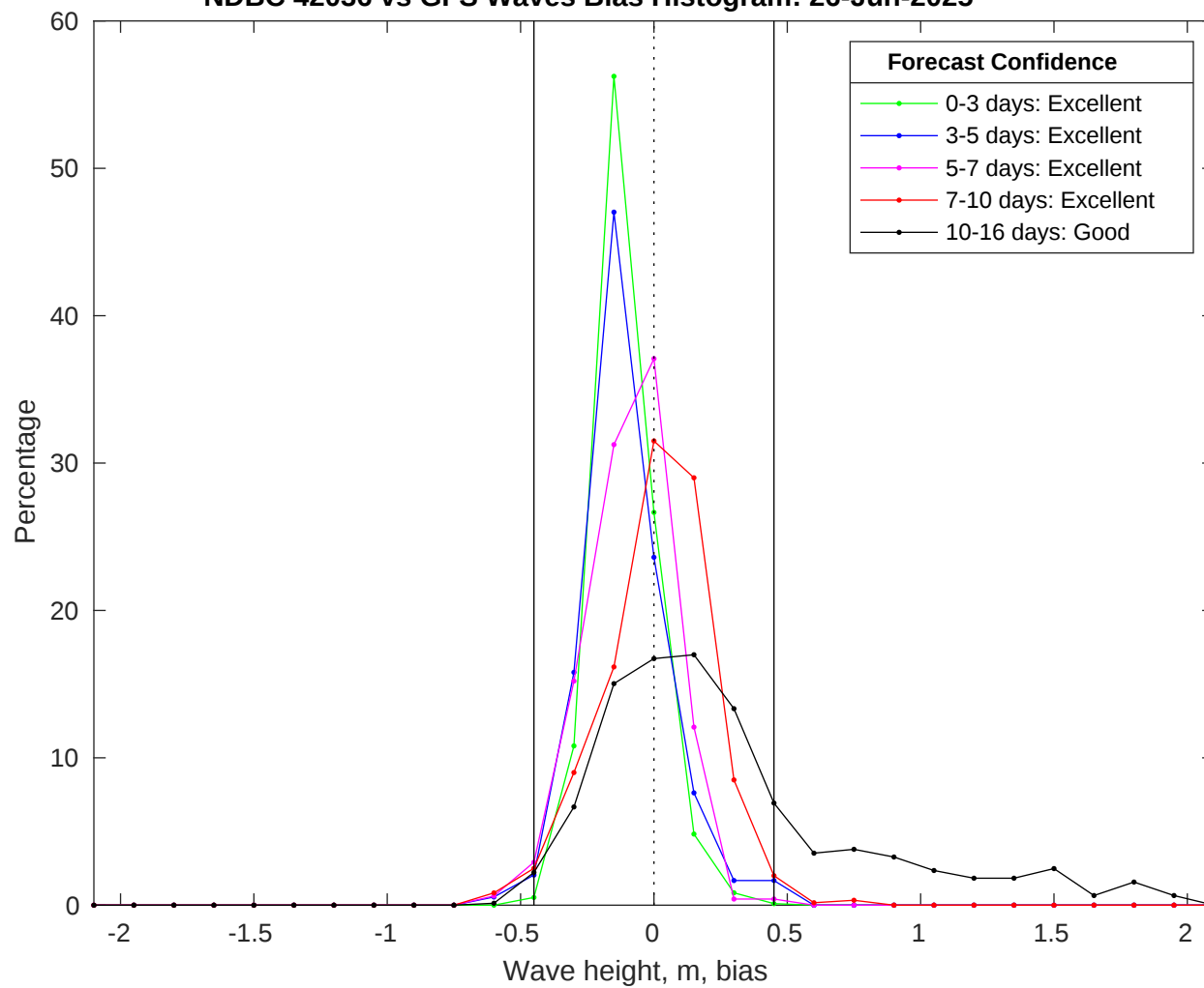
NDBC 42036 vs GFS Waves Bias Histogram: 26-Jun-2025
