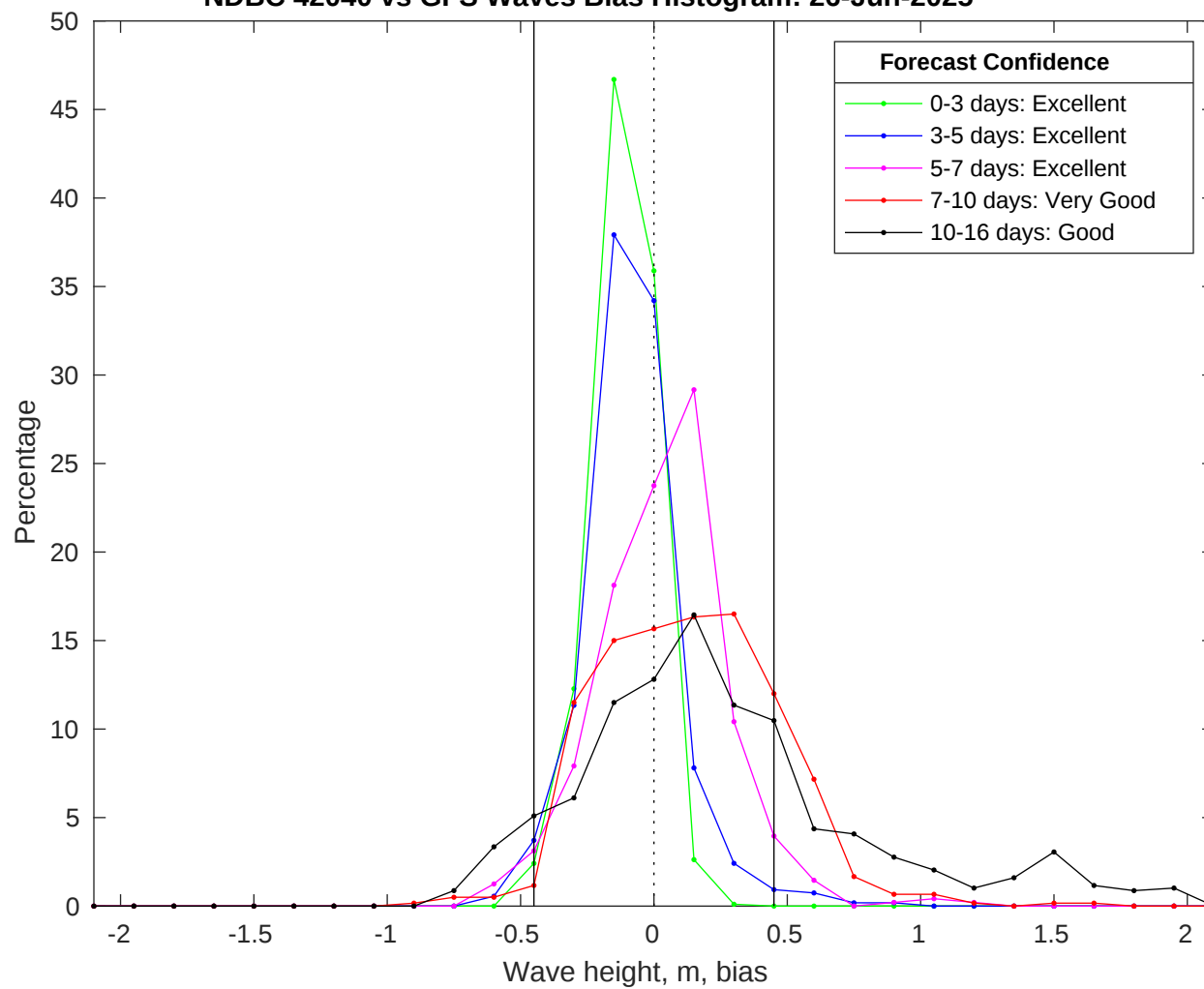
NDBC 42040 vs GFS Waves Bias Histogram: 26-Jun-2025
