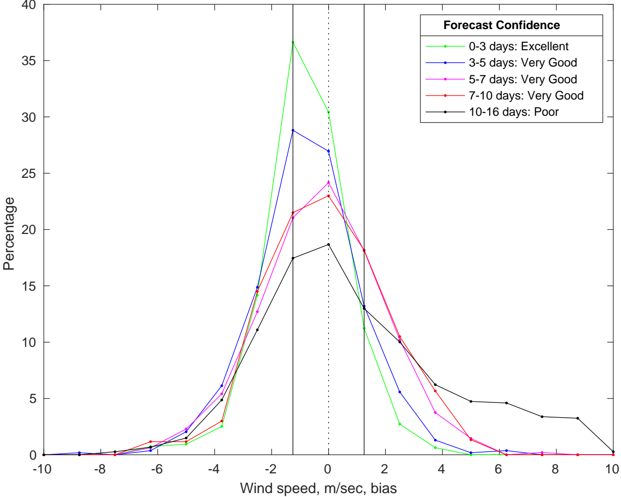
NDBC 42040 vs GFS Winds Bias Histogram: 26-Jun-2025
