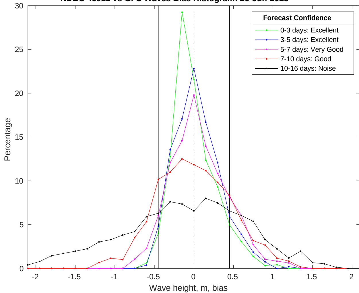
NDBC 46011 vs GFS Waves Bias Histogram: 26-Jun-2025
