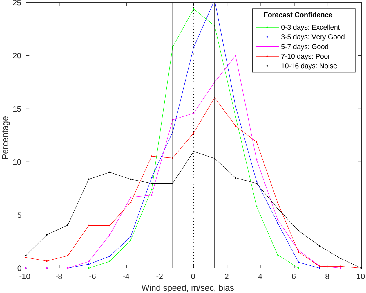
NDBC 46011 vs GFS Winds Bias Histogram: 26-Jun-2025
