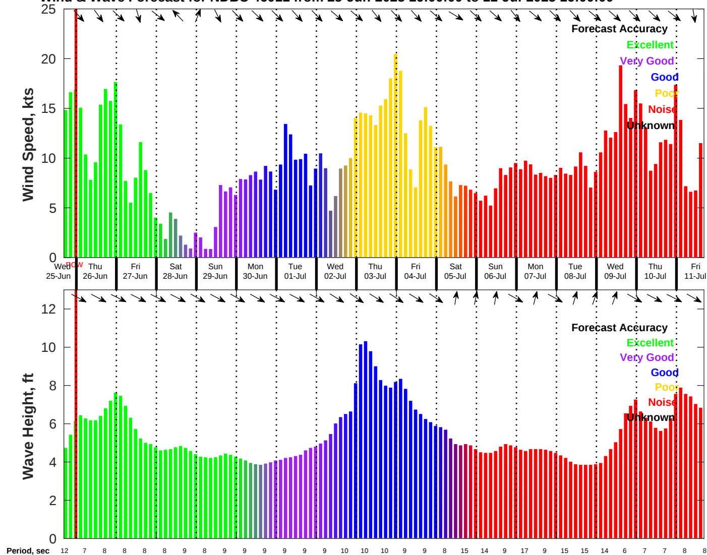
Wind & Wave Forecast for NDBC 46011 from 25-Jun-2025 16:00:00 to 11-Jul-2025 16:00:00
