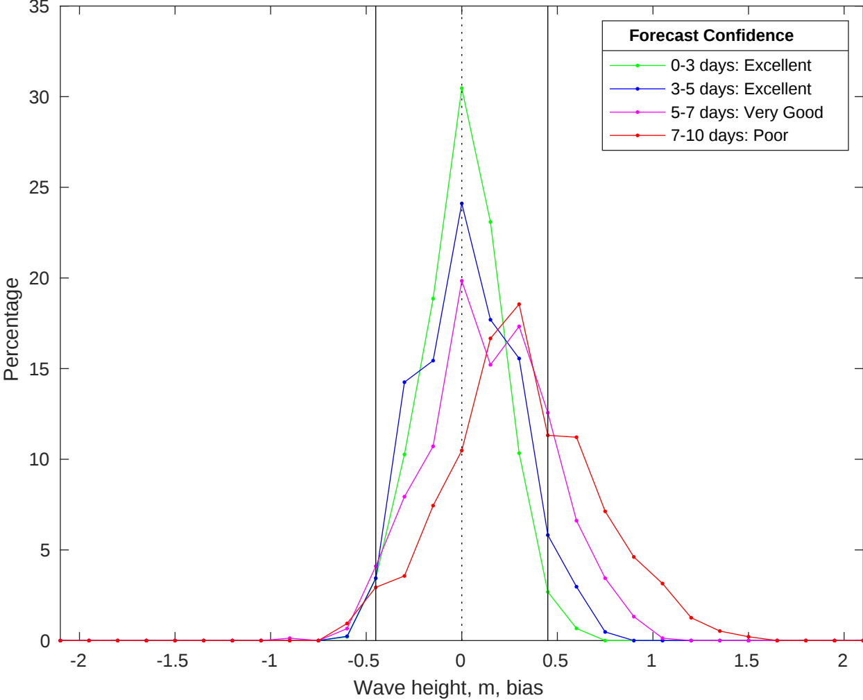
NDBC 46028 vs CMEMS Waves Bias Histogram: 26-Jun-2025
