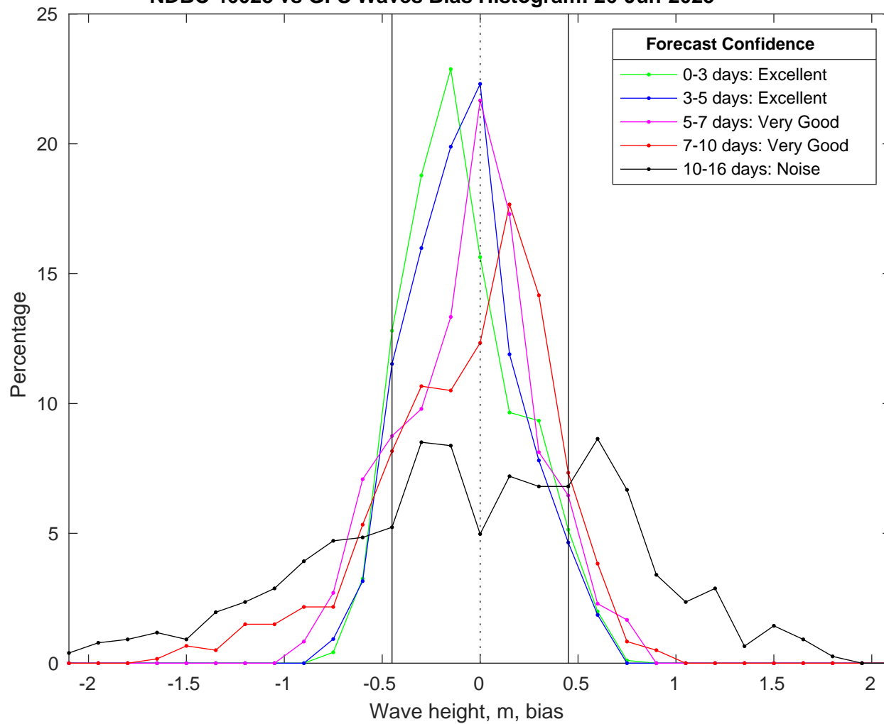
NDBC 46028 vs GFS Waves Bias Histogram: 26-Jun-2025
