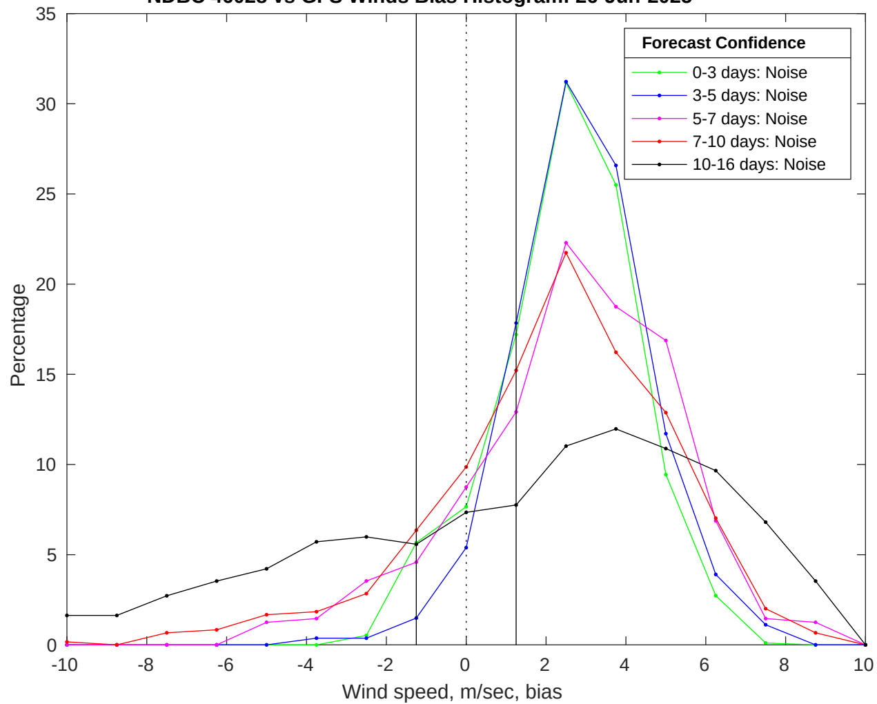
NDBC 46028 vs GFS Winds Bias Histogram: 26-Jun-2025
