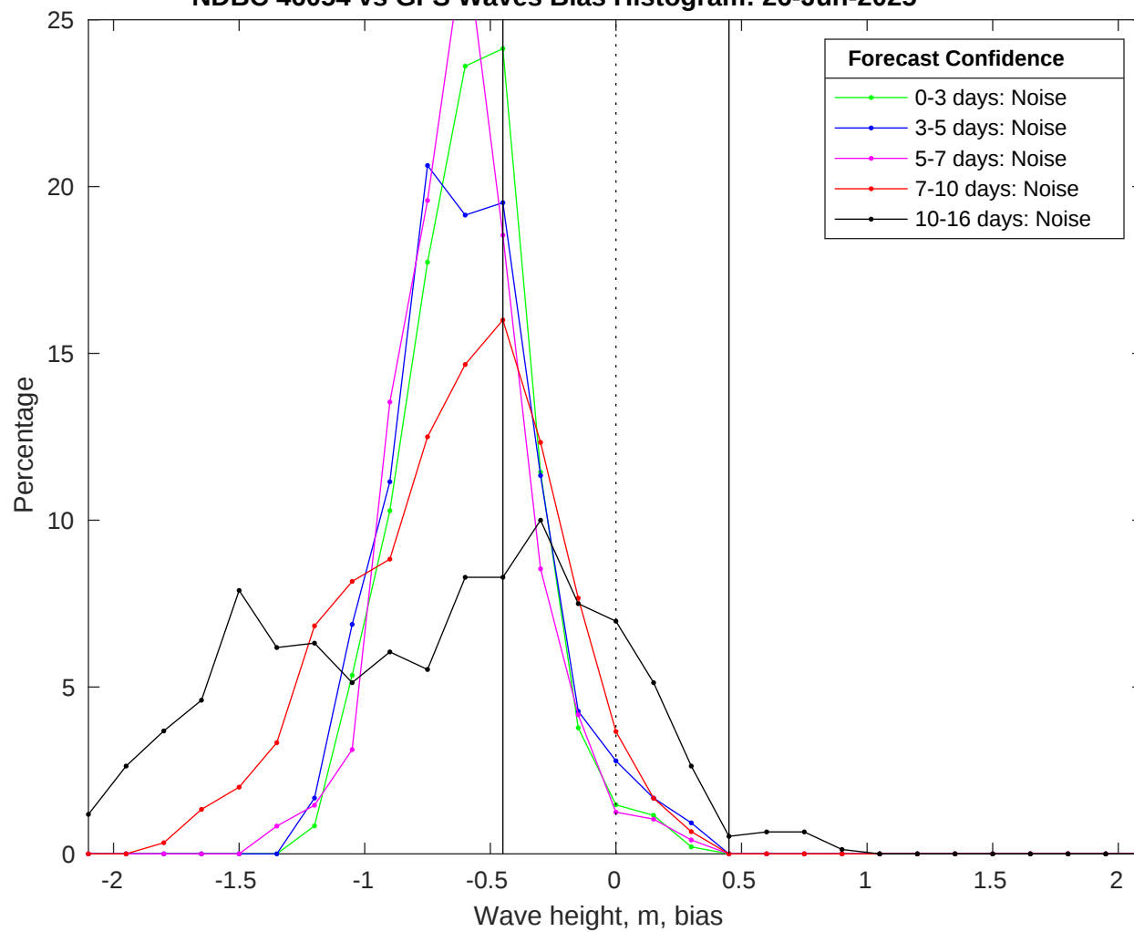
NDBC 46054 vs GFS Waves Bias Histogram: 26-Jun-2025
