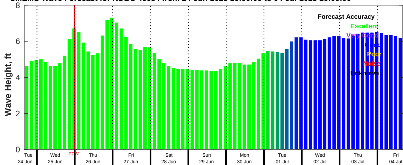
CMEMS Wave Forecast for NDBC 46054 from 24-Jun-2025 16:00:00 to 04-Jul-2025 16:00:00
