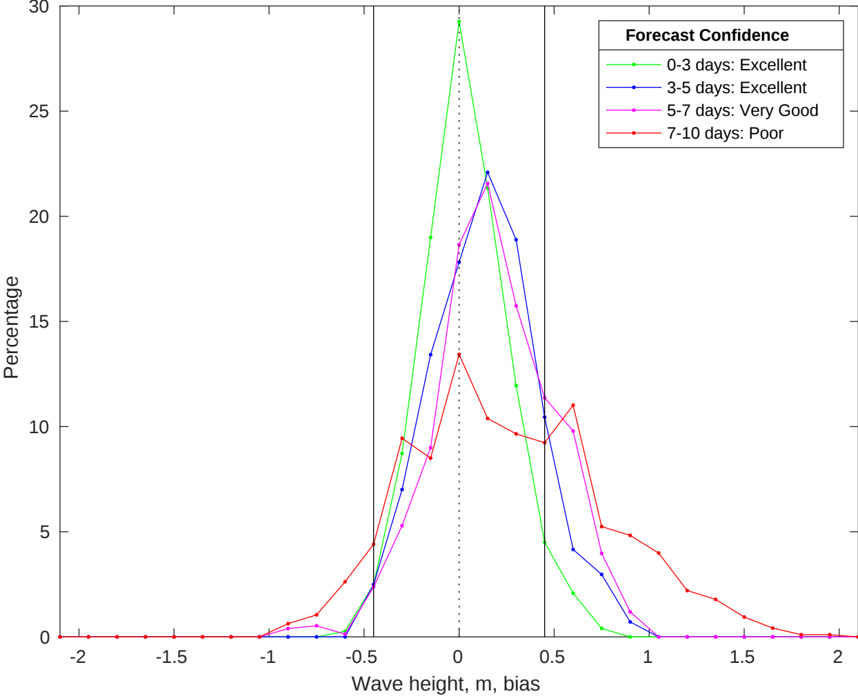
NDBC 46069 vs CMEMS Waves Bias Histogram: 26-Jun-2025
