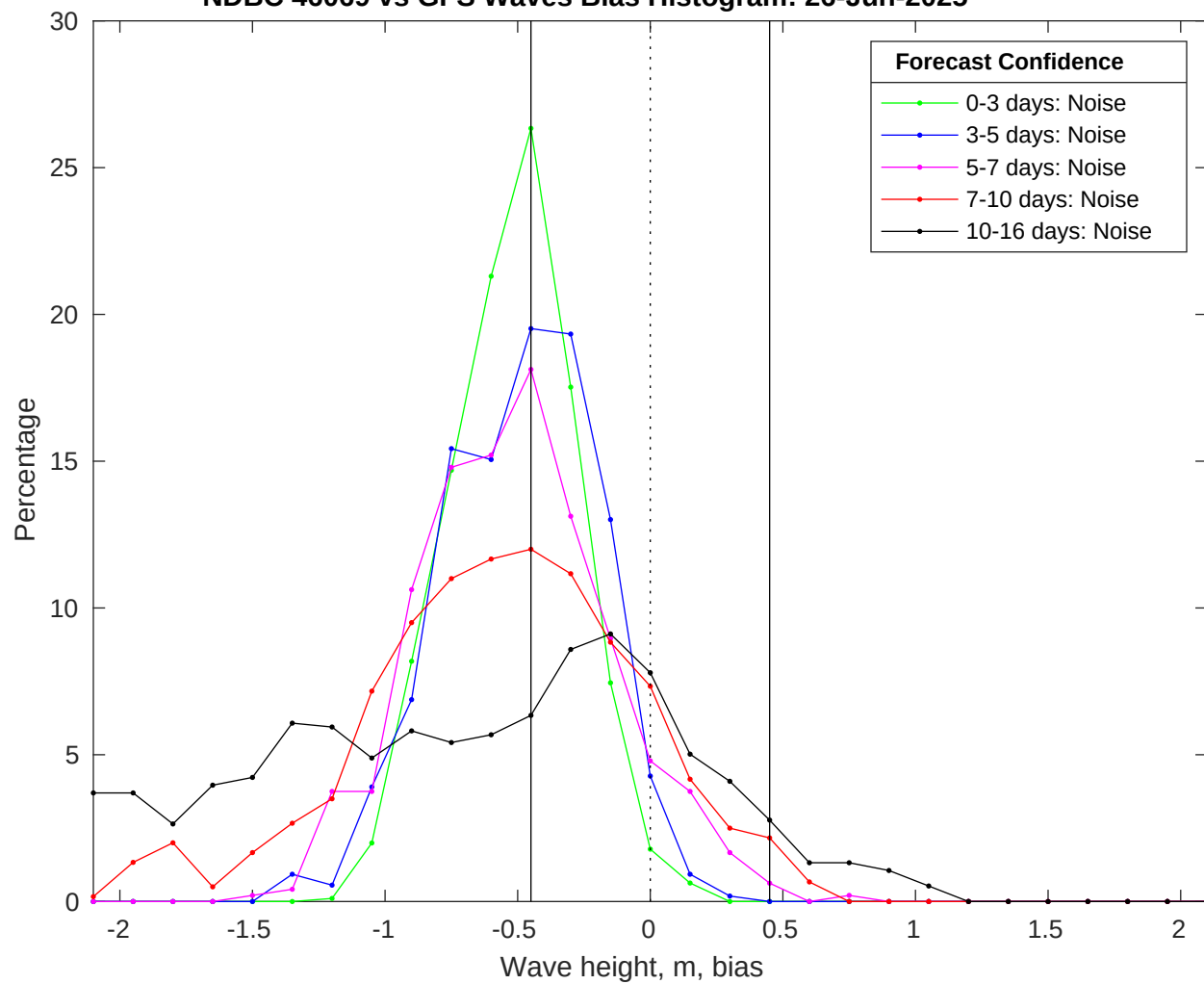
NDBC 46069 vs GFS Waves Bias Histogram: 26-Jun-2025
