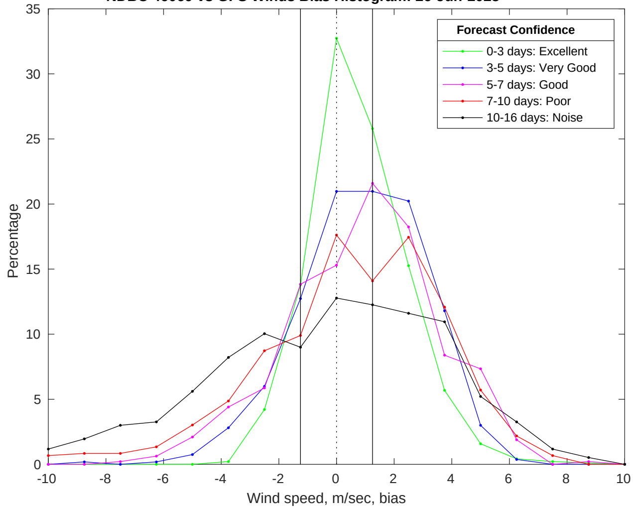
NDBC 46069 vs GFS Winds Bias Histogram: 26-Jun-2025
