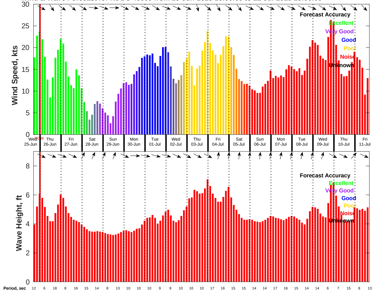
Wind & Wave Forecast for NDBC 46069 from 25-Jun-2025 16:00:00 to 11-Jul-2025 16:00:00
