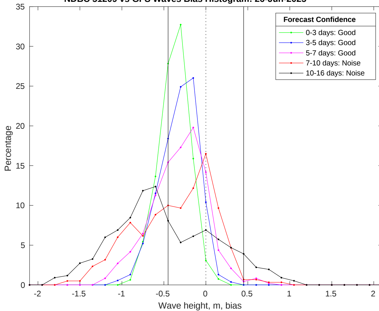
NDBC 51209 vs GFS Waves Bias Histogram: 26-Jun-2025
