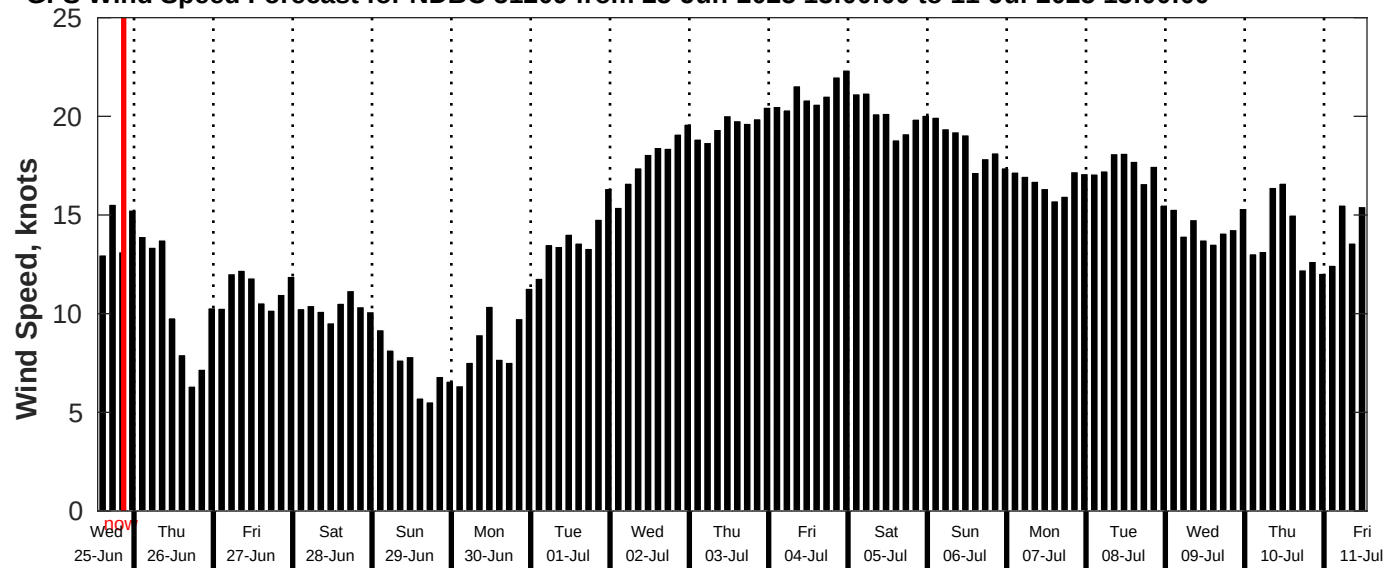
GFS Wind Speed Forecast for NDBC 51209 from 25-Jun-2025 13:00:00 to 11-Jul-2025 13:00:00
