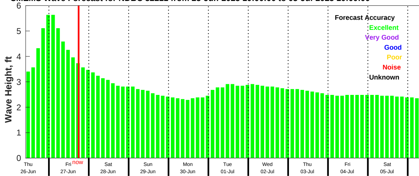
CMEMS Wave Forecast for NDBC 52211 from 25-Jun-2025 10:00:00 to 05-Jul-2025 10:00:00
