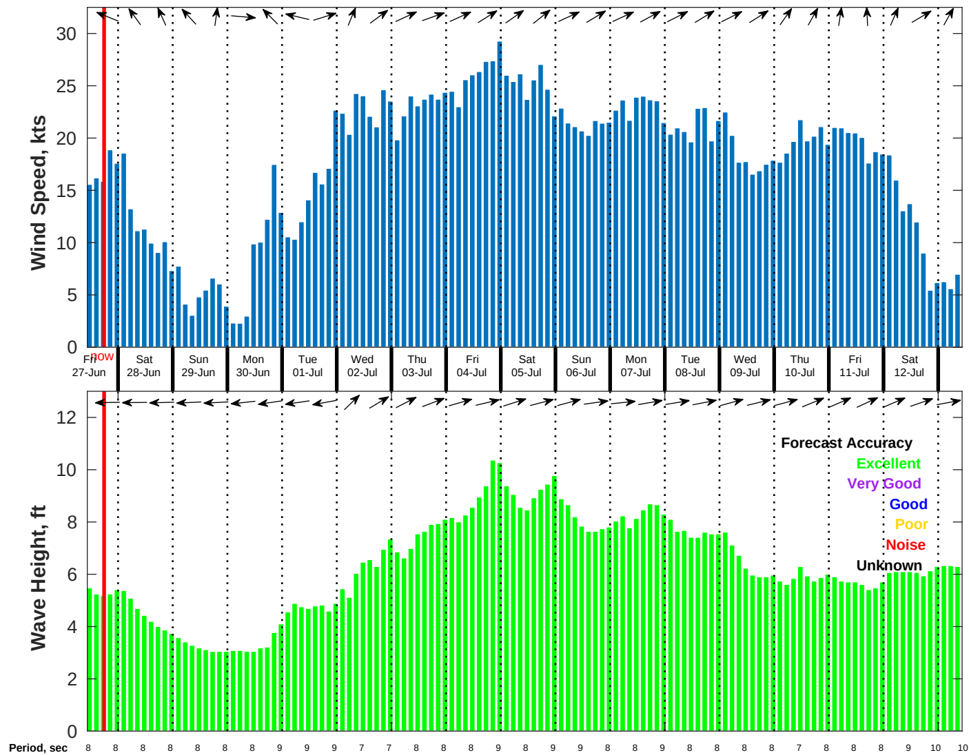
Wind & Wave Forecast for NDBC 52211 from 26-Jun-2025 10:00:00 to 12-Jul-2025 10:00:00
