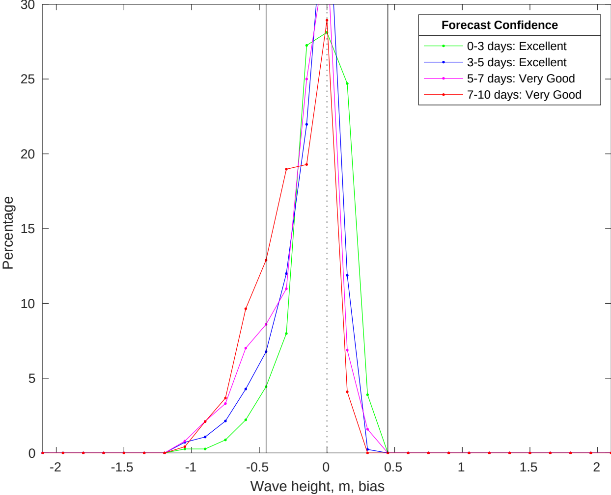
NDBC 52212 vs CMEMS Waves Bias Histogram: 26-Jun-2025
