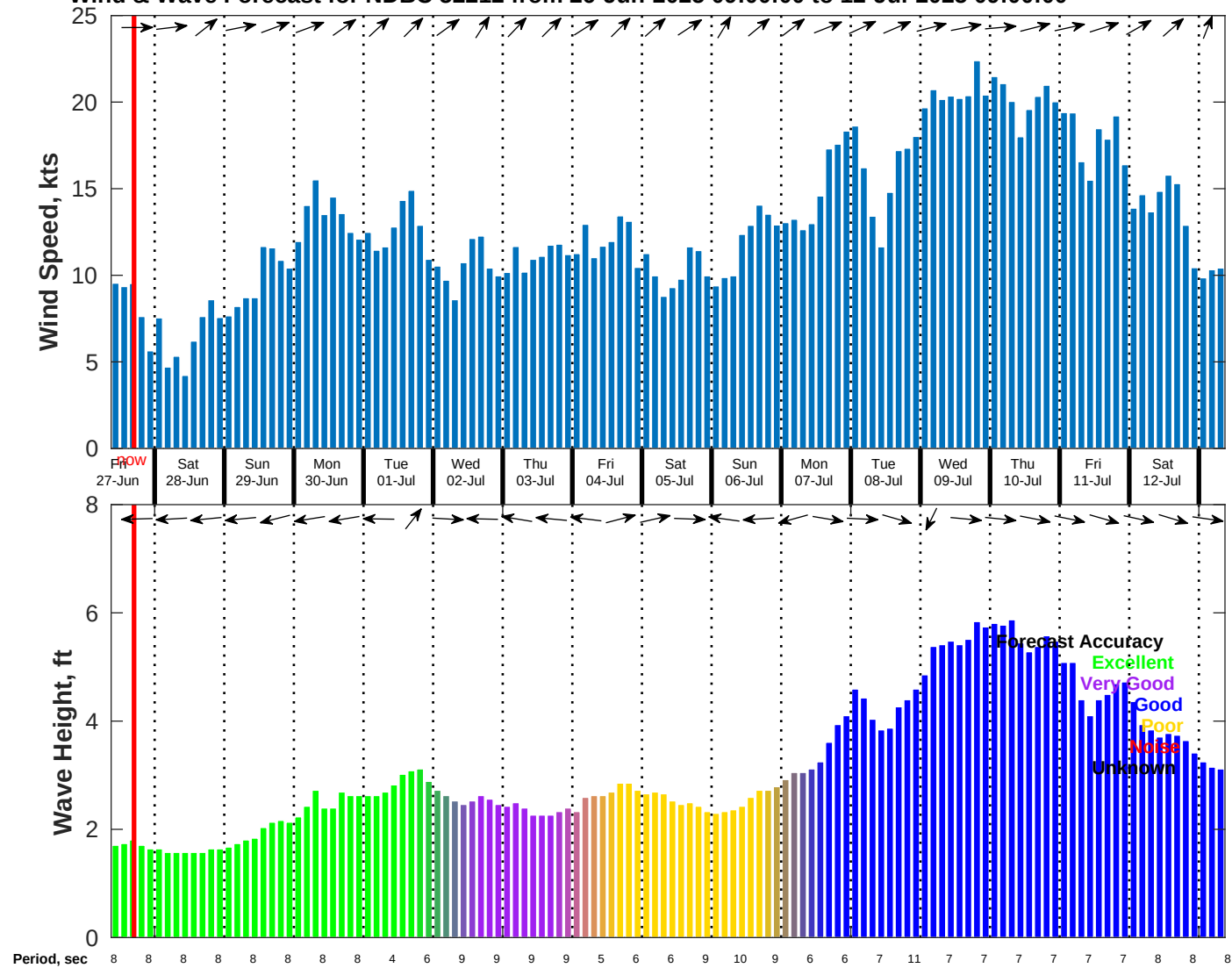
Wind & Wave Forecast for NDBC 52212 from 26-Jun-2025 09:00:00 to 12-Jul-2025 09:00:00
