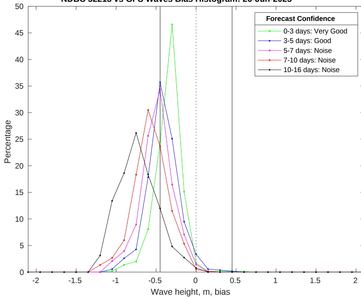
NDBC 52213 vs GFS Waves Bias Histogram: 26-Jun-2025
