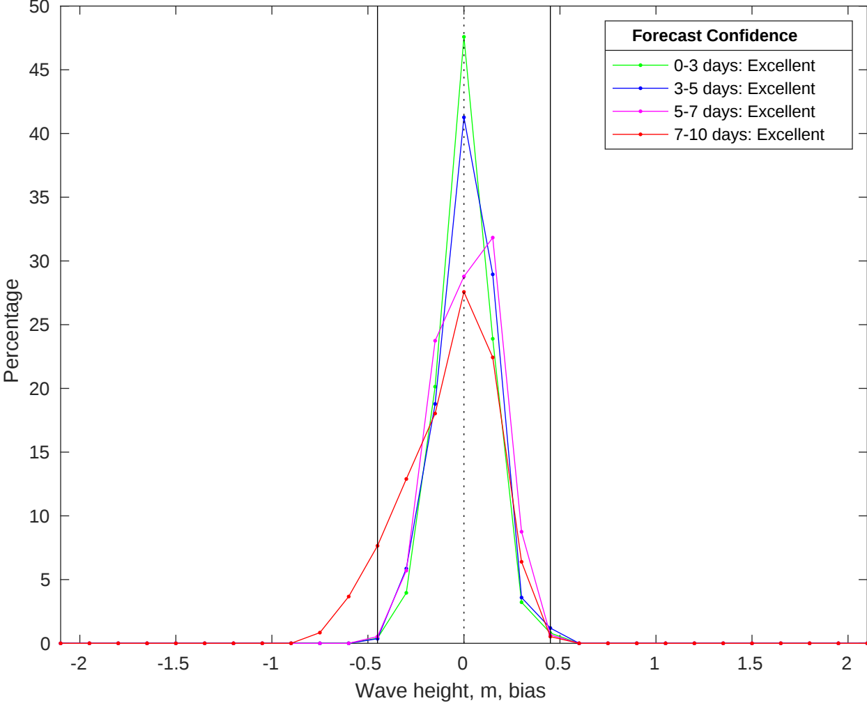
NDBC 41004 vs CMEMS Waves Bias Histogram: 27-Jun-2025
