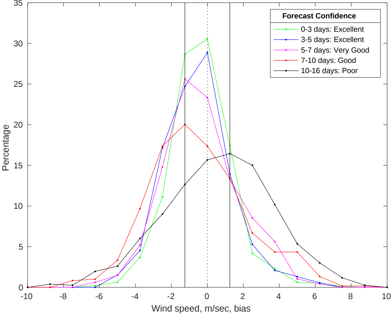
NDBC 41004 vs GFS Winds Bias Histogram: 27-Jun-2025
