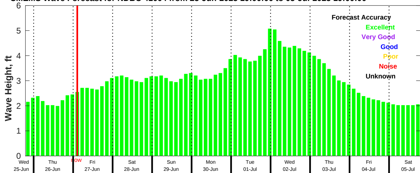
CMEMS Wave Forecast for NDBC 41004 from 25-Jun-2025 19:00:00 to 05-Jul-2025 19:00:00
