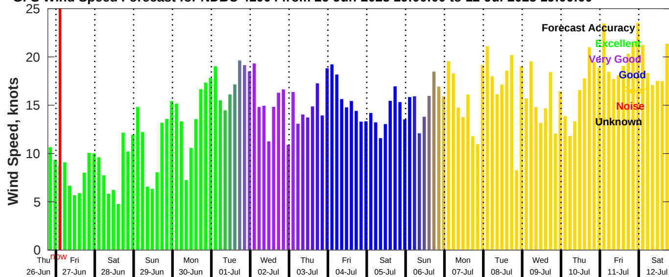
GFS Wind Speed Forecast for NDBC 41004 from 26-Jun-2025 19:00:00 to 12-Jul-2025 19:00:00
