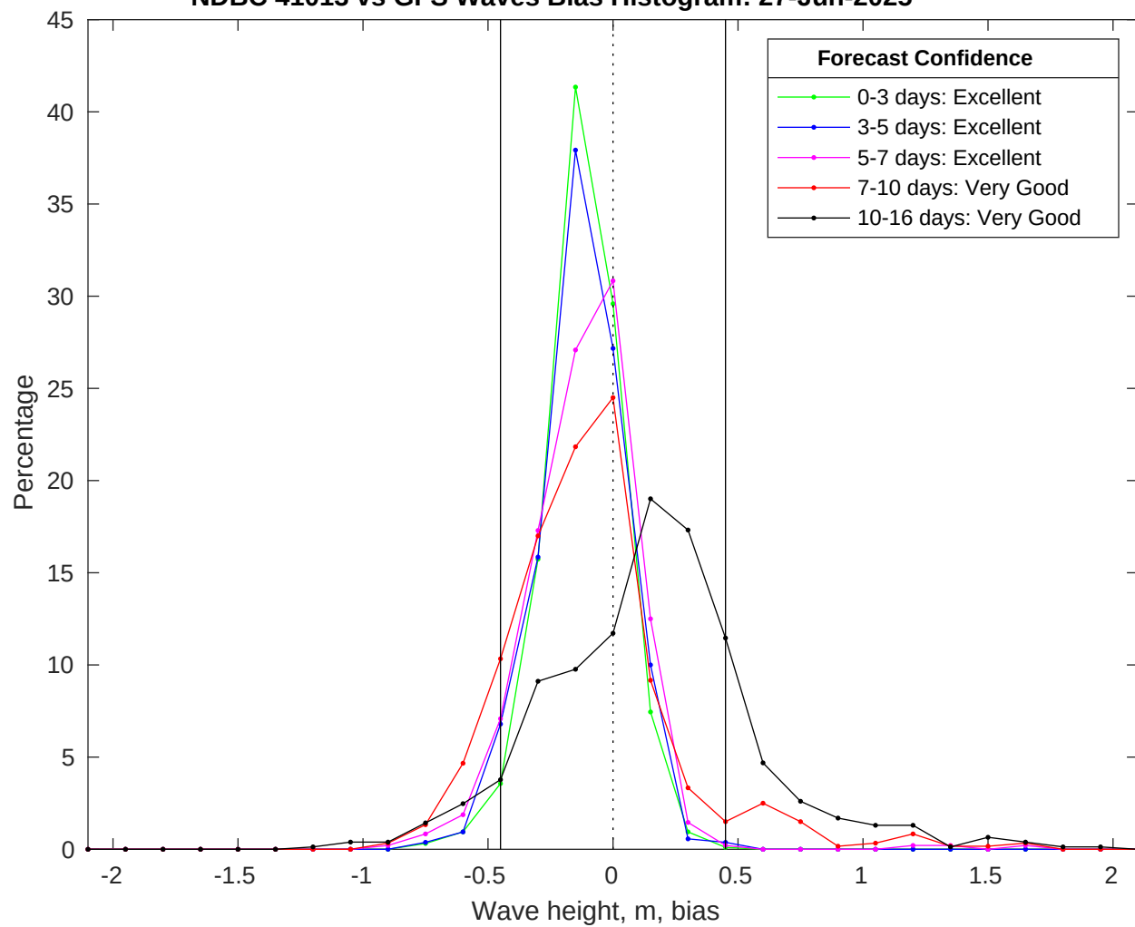
NDBC 41013 vs GFS Waves Bias Histogram: 27-Jun-2025
